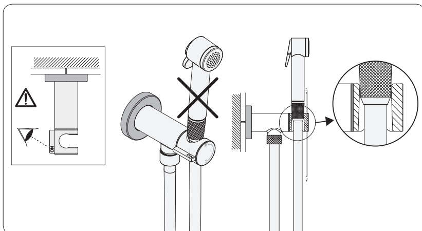
Mixer CLOSE/OFF
